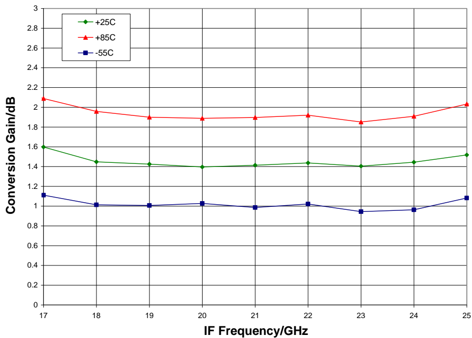
IF Bandwidth, LO = +2 dBm, T_A = 25^\circ\text{C}
