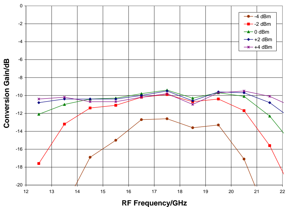
Upconverter Performance, Conversion Gain vs. LO Drive, T_A = 25^\circ\text{C}
