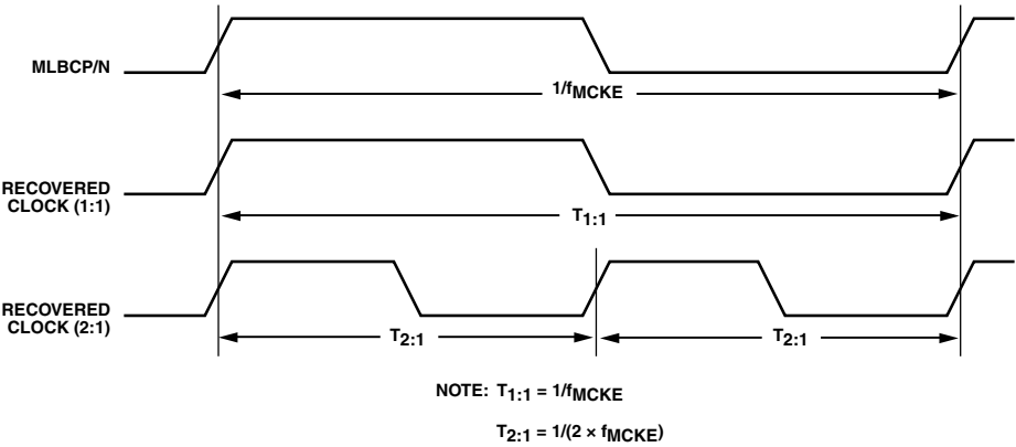
Figure 52. MLB 6-Pin Clock Definitions
