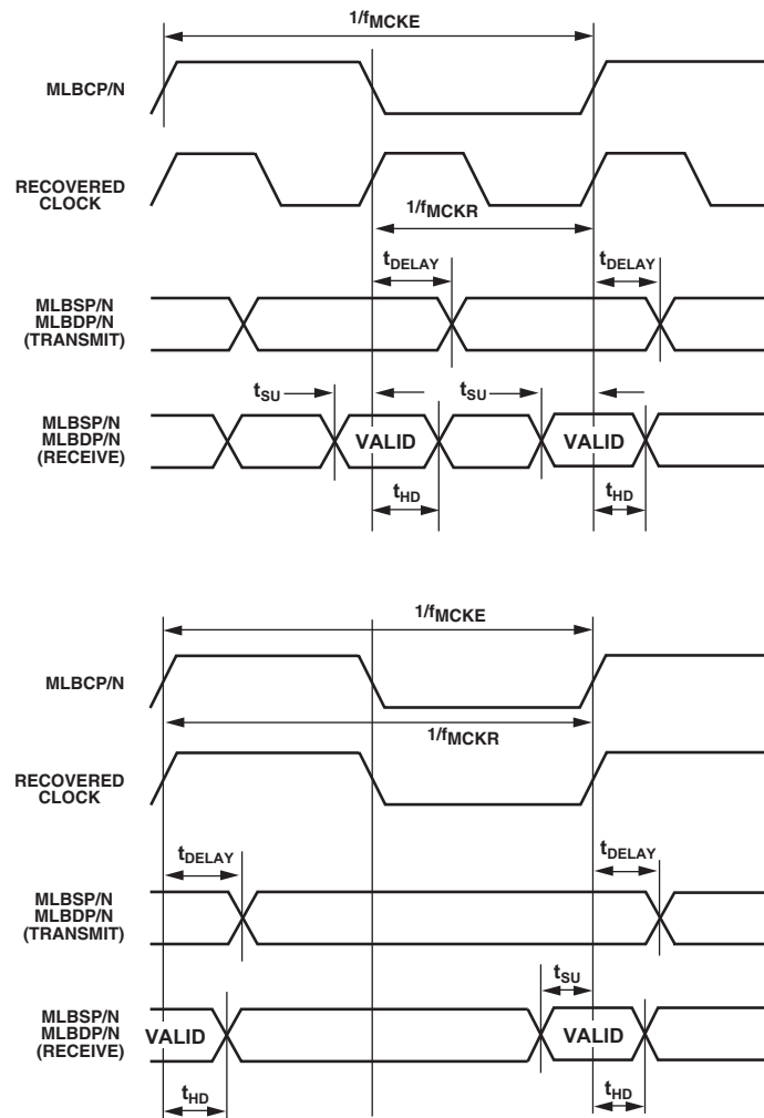
Figure 53. MLB 6-Pin Delay, Setup, and Hold Times
