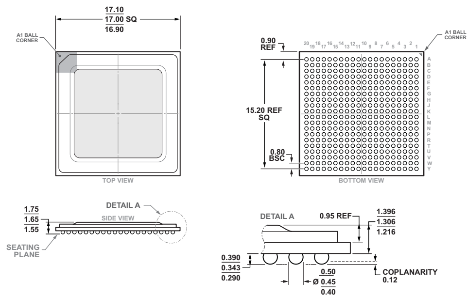
Figure 72. 400-Ball Ball Grid Array, Thermally Enhanced [BGA_ED] (BP-400-2) Dimensions shown in millimeters
