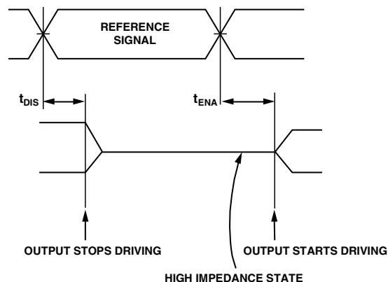
Figure 64. Output Enable/Disable
