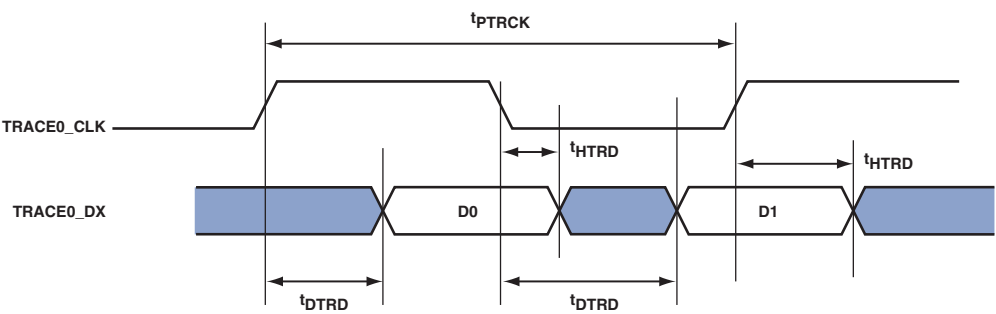
Figure 55. Trace Timing
