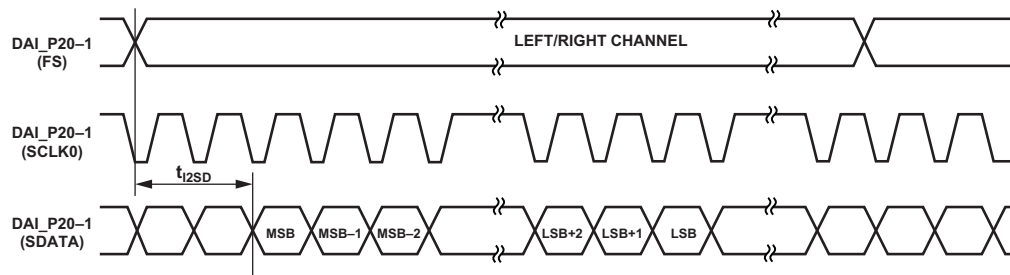
Figure 46. I 2 S Justified Mode
