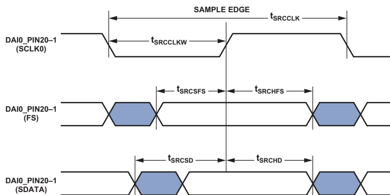
Figure 17. ASRC Serial Input Port Timing
