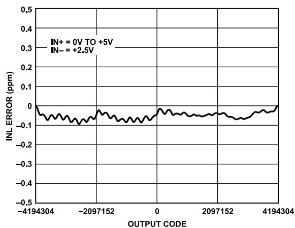
Figure 13. INL vs. Output Code, Single-Ended Input
