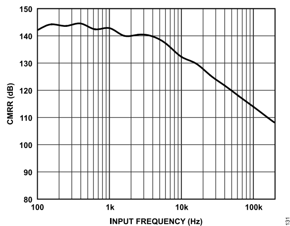
Figure 30. Common-Mode Rejection Ratio (CMRR) vs. Frequency
