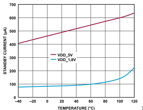
Figure 34. Supply Standby Current vs. Temperature
