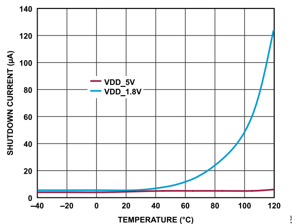
Figure 35. Supply Shutdown Current vs. Temperature
