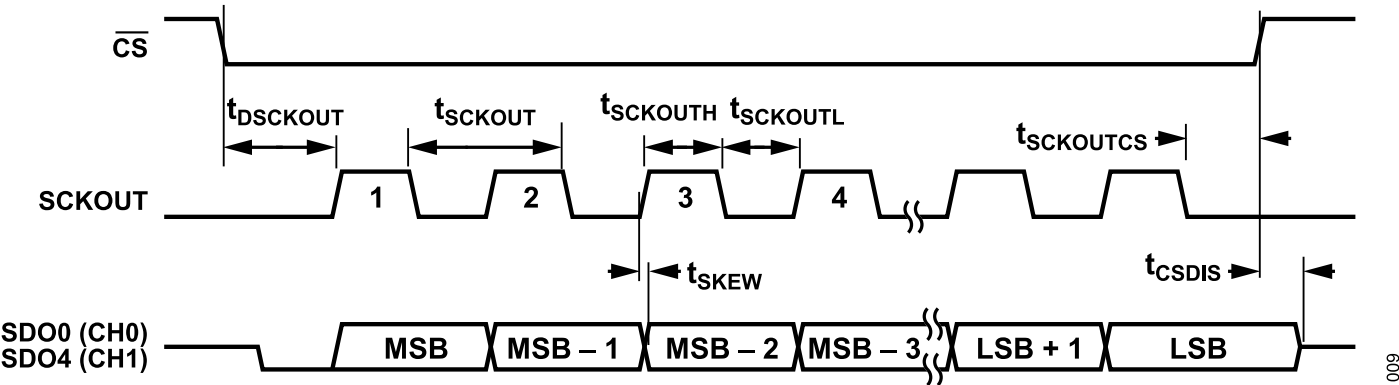
Figure 9. Master Clock Mode Timing, SDR, 1-Lane
