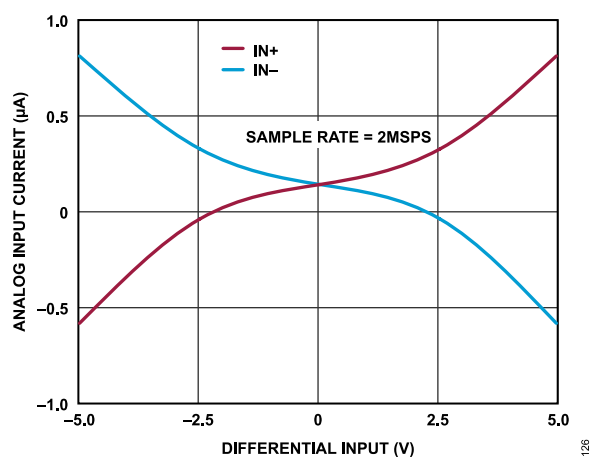
Figure 25. Analog Input Current vs. Differential Input
