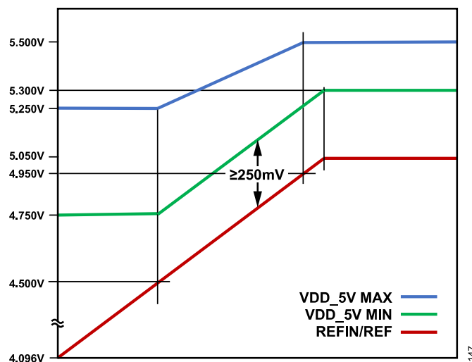
Figure 45. \text{VDD\_5V} Minimum and Maximum Values for \text{REFIN/REF}
