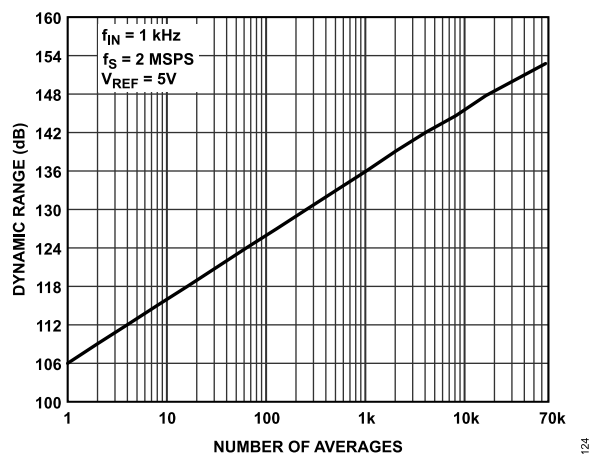
Figure 23. Dynamic Range vs. Averaging
