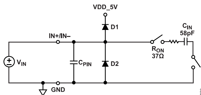
Figure 38. Equivalent Circuit for the AD4630-24 Differential Analog Input
