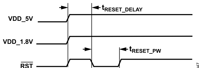
Figure 44. Power-On Reset (POR) Timing
