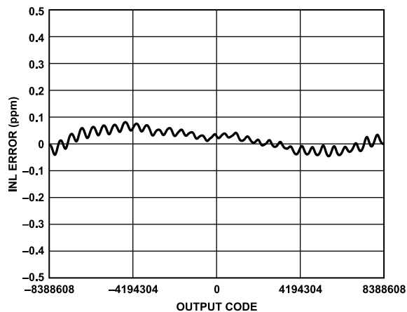
Figure 12. INL vs. Output Code, Differential Input
