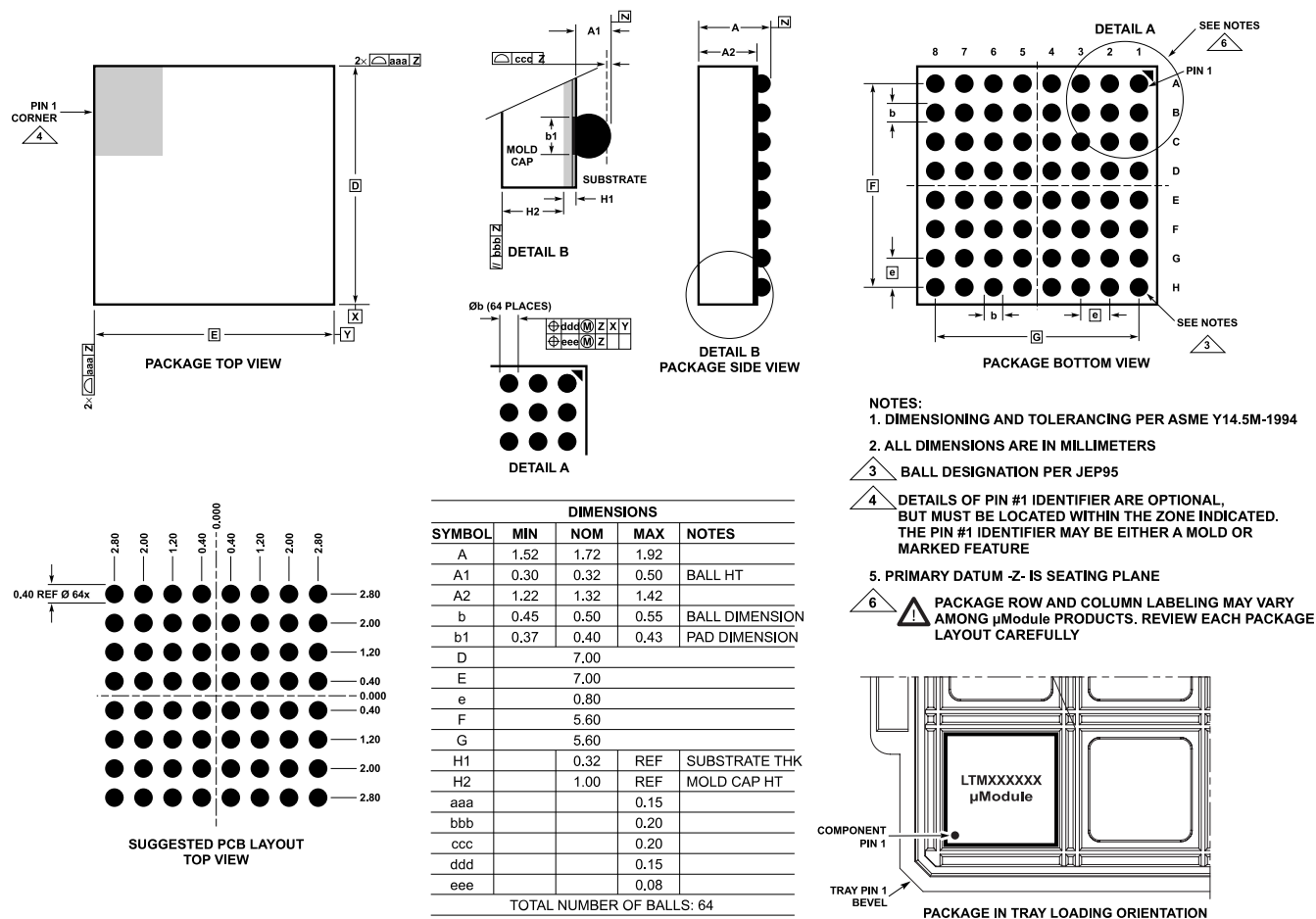
Figure 57. 64-Ball Chip Scale Package Ball Grid Array [CSP_BGA] (BC-64-8)
