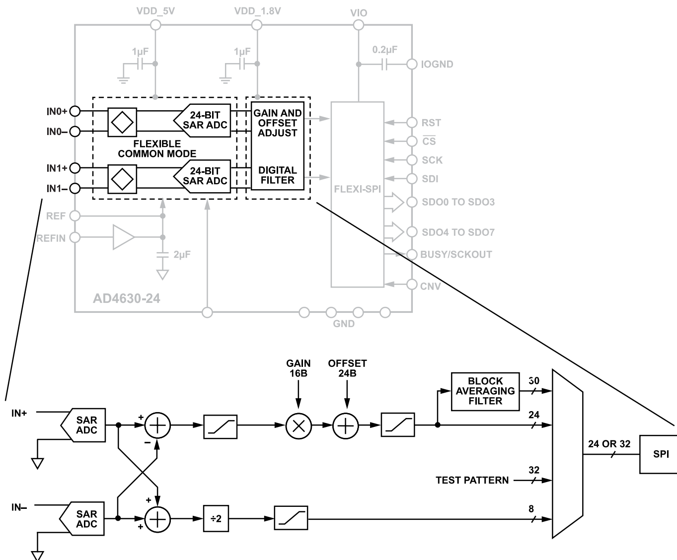
Figure 36. AD4630-24 Functional Block Diagram and Channel Architecture
