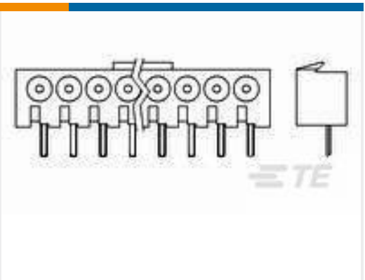
TE 产品编号1888290-6 .100 SRRA T-H, Latchg Flexstrip Recep
