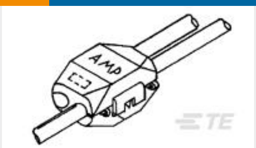
TE 产品编号171404-1 ELECTRO TAP 14-16
