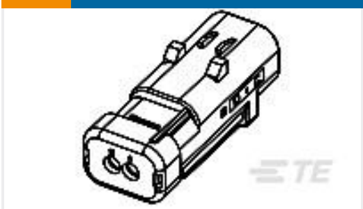
TE 产品编号1717672-3 CAP ASSY,2P,BRACKET REVERSE TYPE,ATAC CO
