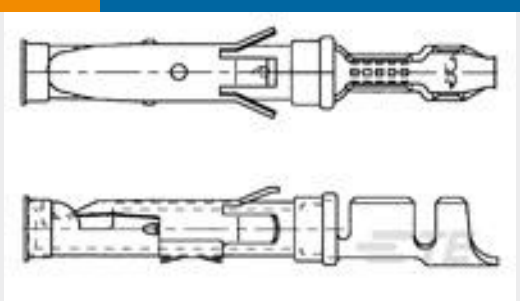
TE 产品编号1-163084-0 SPEC. PLATED
