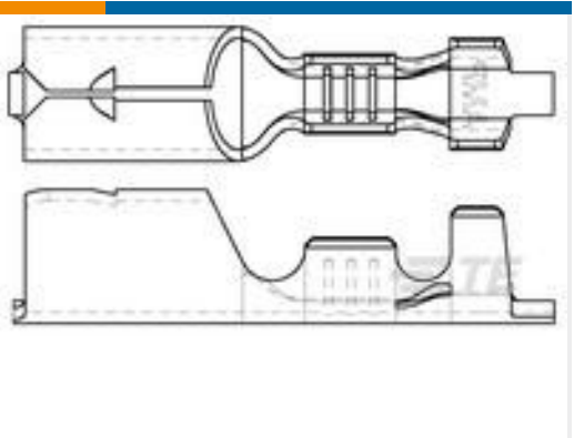
TE 产品编号881724-1 .156 DIA SHUR PWG R
