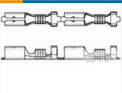
TE 产品编号626399-2 .140 SHUR PLUG REC.
