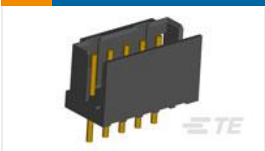
TE 产品编号1-292133-4 CT P/HDR ASSY BOX V 14P W/O KI
