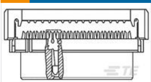
TE 产品编号1-1546310-0 10P.563" DR BARRIER STRIP
