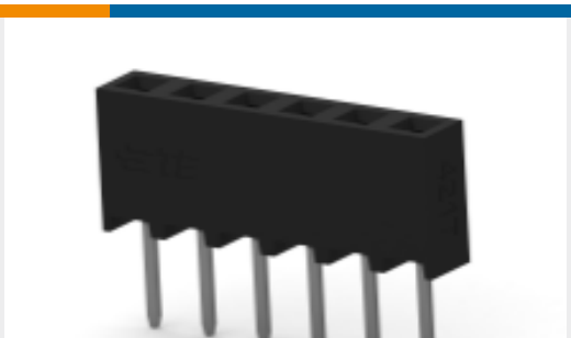
TE 产品编号2314878-6 6P, 2MM, B-B, REC, SRVT, 2.7, 0.76AU, TB
