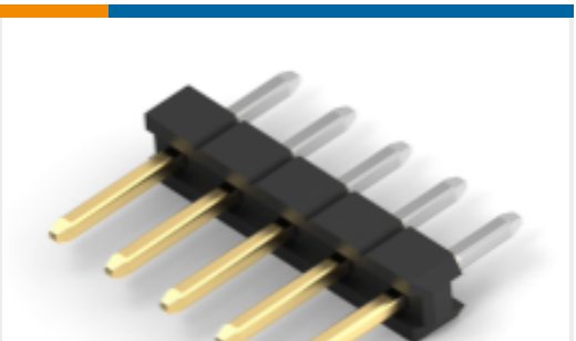
TE 产品编号2355045-6 6P, 2MM, BRK HDR, SRVT, 2.8, 0.1AU, TB
