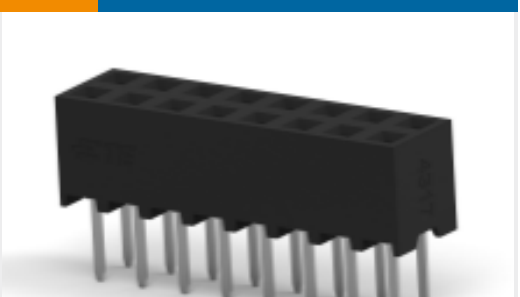
TE 产品编号1-2314826-6 16P,2MM,B-B,REC,DRVT,2.7,0.76AU, TB,W/CAP
