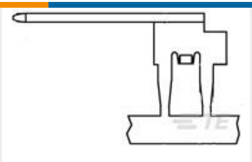
TE 产品编号1217089-1 110 FASTON,PCB TAB,TNBR
