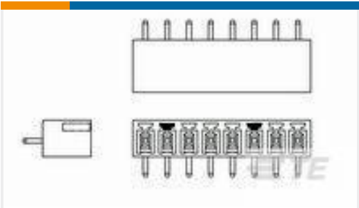
TE 产品编号1776553-8 Vert Header, Green, 3.81mm, Keyed
