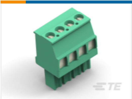
TE 产品编号 1986375-2 Str Plug, 3.81mm, Green, LH, 2
