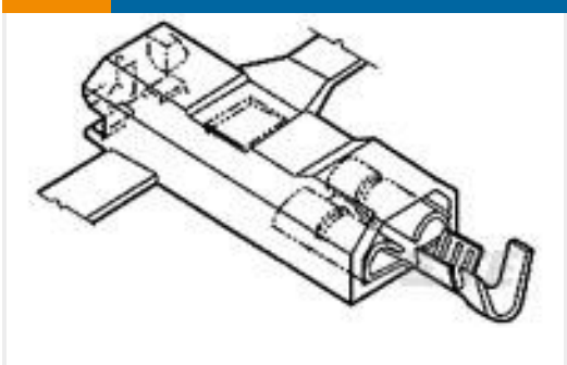
TE 产品编号1969206-1 ULTRA-POD .250 ASSEMBLY REC 18-14 AWG BR
