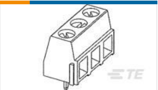
TE 产品编号2-282837-4 TERMI-BLOK PCB MOUNT 24P
