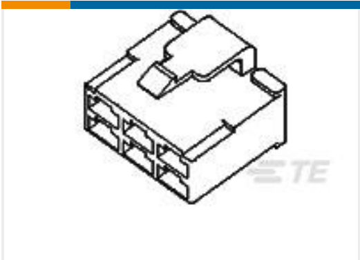
TE 产品编号171898-2 FF 250 PLUG HSG 6P NYLON BLACK
