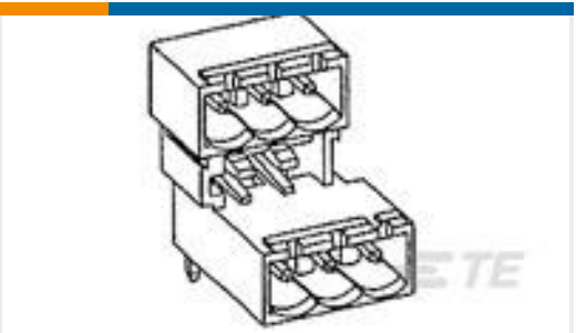
TE 产品编号284061-3 TERMI-BLOK HDR 90, 5,08MM P. M
