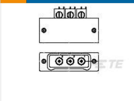
TE 产品编号1589072-9 CX050L2HN = COAX
