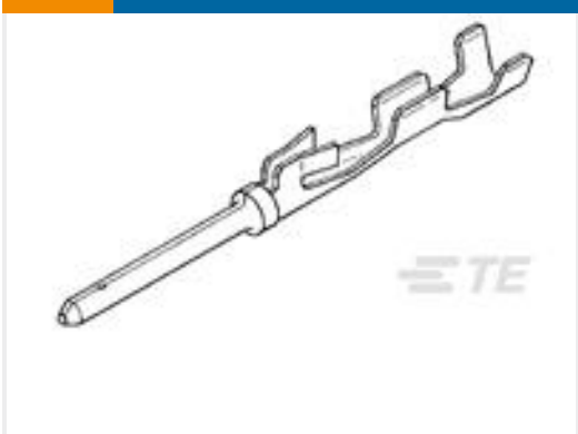
TE 产品编号1-745266-0 PIN CONTACT,HDE-20,#22-26 AWG
