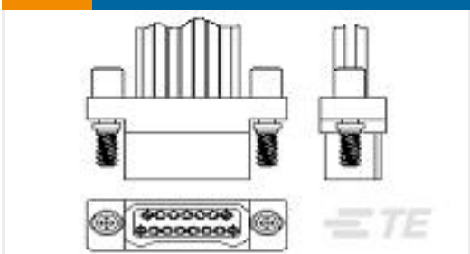
TE 产品编号6-1589473-0 STM015PC2DT012N = WDUALOB
