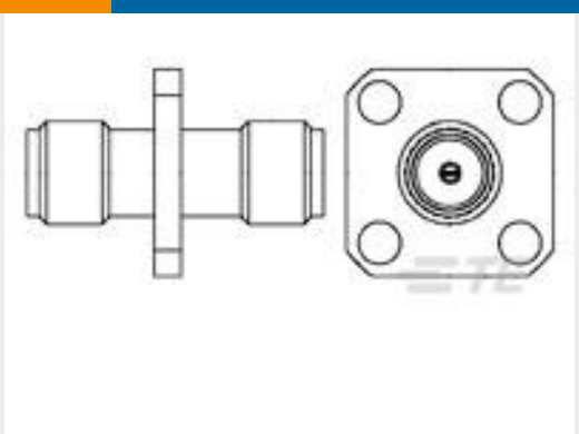
TE 产品编号1054988-1 SMA Jack-Jack Adapter 2084 8002 92
