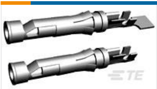
TE 产品编号1-66358-0 III+ SKT,18-14,30AU/FL,STRIP
