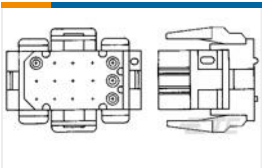
TE 产品编号1-640519-0 04P MR II PLUG HSG V0 RED
