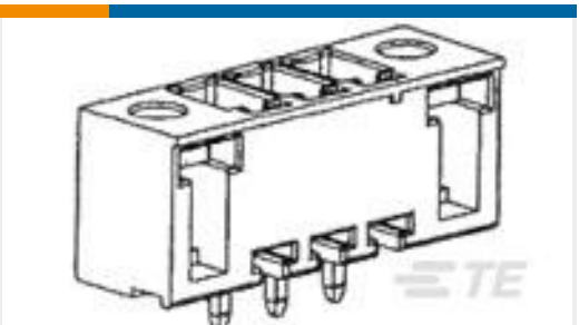
TE 产品编号284519-4 4P TERMIBLOK HDR DIR VITI 3
