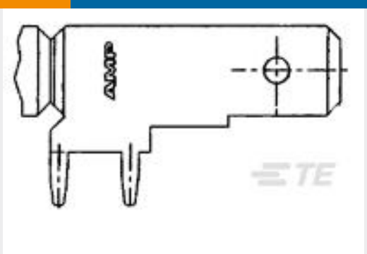
TE 产品编号1217754-1 250 FASTON,FLAG,PCB TAB,TNBR
