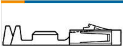
TE 产品编号1-104480-7 SHORT POINT CONT PLTD SN
