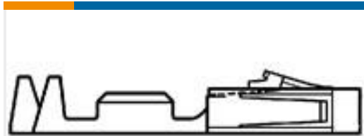
TE 产品编号1-104480-3 SHORT POINT CONT 30 DPLX STMPD LF
