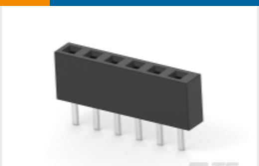
TE 产品编号1834039-6 Header Recp., 2mm, 6 POS, GOLD FLASH
