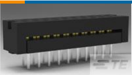
TE 产品编号1-746610-8 34 DIP PLUG, 100CL, LEAD FREE
