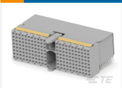
TE 产品编号3-646486-0 8-ROW,TWST,TUL TYPE/D W/SHEILD
