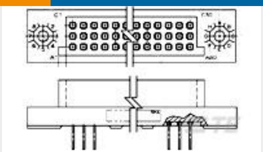
TE 产品编号448005-1 3 ROW BOX RECP 180 POS 100C/L
