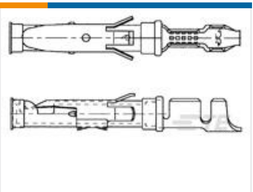
TE 产品编号163087-9 062 SOC.ASS. TYP3+
