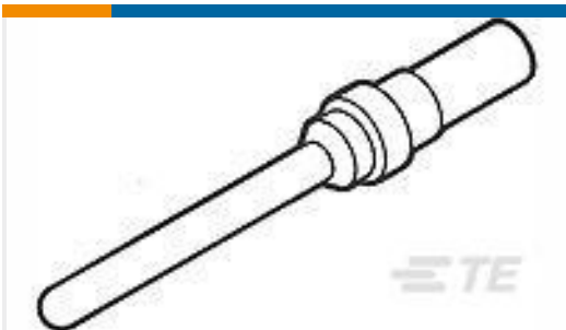
TE 产品编号1218266-1 CONT,CRIMP PIN,18AWG,109,SZ 20
