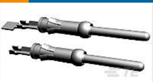
TE 产品编号1-66103-4 III+ PIN,24-20,30AU>10,SMPACK
