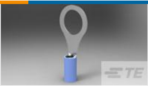
TE 产品编号2-320575-1 TERMINAL,PIDG R 16-14 5/16
