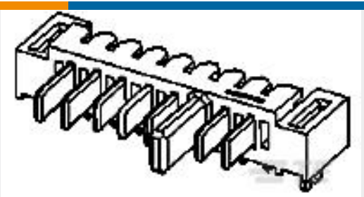
TE 产品编号1932154-1 2mm pitch Battery Plug Assy.7Pos Reverse
