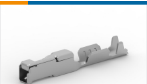
TE 产品编号2035170-8 CONTACT,FEMALE, 0.64, 0.35SQMM, CUNISI
