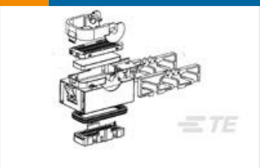
TE 产品编号368434-1 ECU 64P CONN ASSY(32bit-M)BLK
