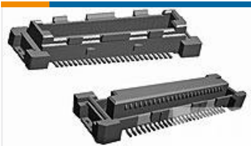
TE 产品编号 1-5353188-0 .6FHP08H,140,S,GIG,08/Sn,TR,NSYes
