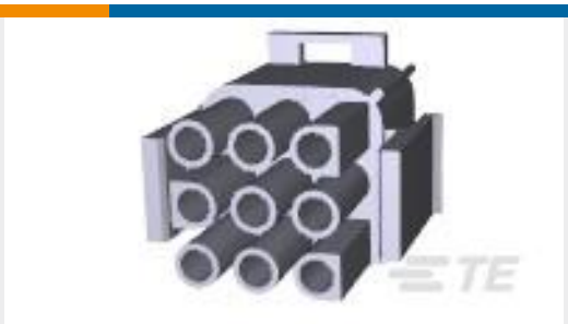
TE 产品编号1-480706-9 09P UMNL PLUG HSG BLK
