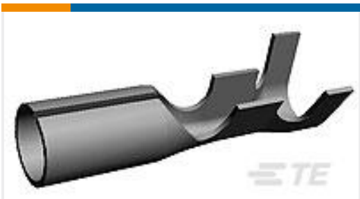
TE 产品编号170021-1 SHUR PLUG RECEPTACLE 20-16 AWG TPBR
