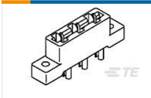
TE 产品编号145340-1 HI CURRENT ASSY 12 POS/8 LOAD
