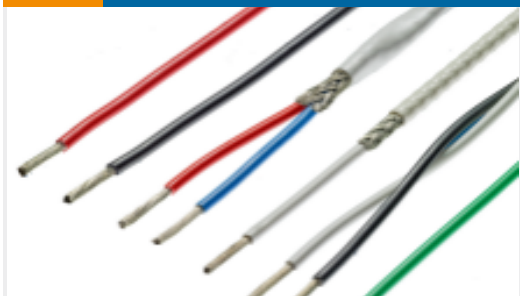
TE 产品编号709517-000 81044/9-12-2
