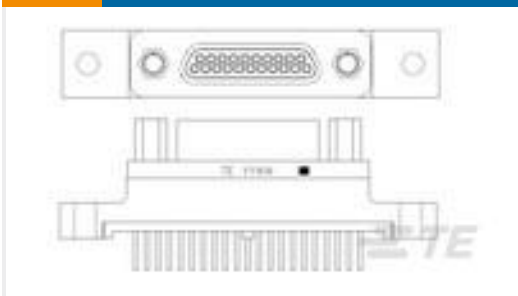
TE 产品编号1532268-3 M83513/22-C01NN = MCKS-N1-B-21PST1
