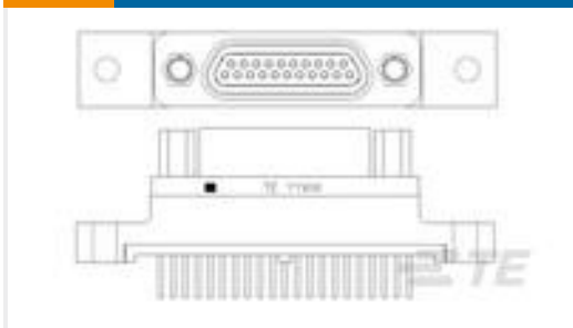
TE 产品编号1532276-3 M83513/25-C01NN = MCKS-N1-B-21SST1
