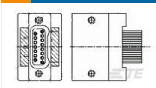
TE 产品编号2-1589488-7 STM015M5PQ = THRU-HOLE
