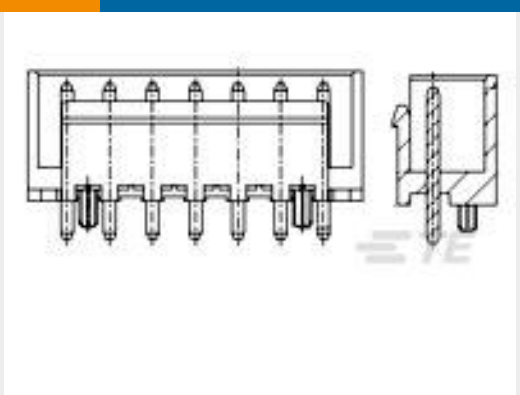
TE 产品编号1744357-3 3.96 EP SHROUDED HDR ASSY 3P W
