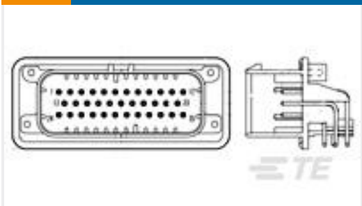
TE 产品编号1-776163-5 HEADER ASSY 35 POS W/GASKET
