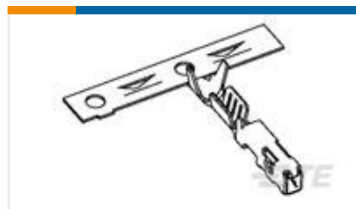
TE 产品编号1924955-1 CONTACT, FEMALE 0.64, 20-22AWG, UNSEAL
