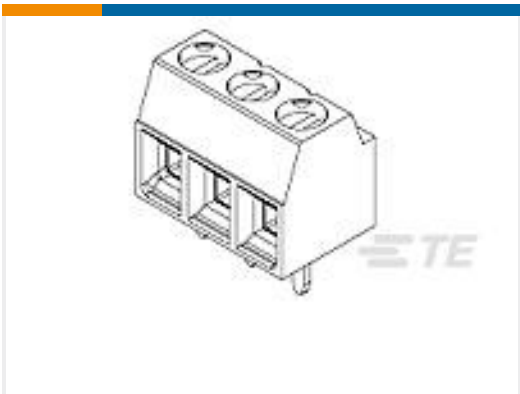
TE 产品编号1776113-3 3P,3.81MM,SIDE ENTRY,HIGH TMP
