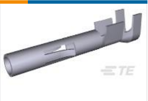
TE 产品编号350550-6 UMNL SOK 20-14 AU/PHBZ L/P
